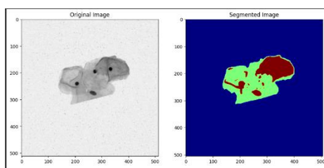
K-Means: Figure 3
