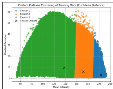
K-Means : Figure 1
