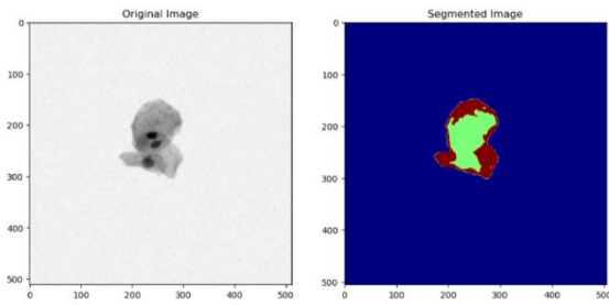
K-Means: Figure 7
