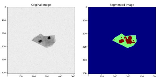
K-Means: Figure 5
